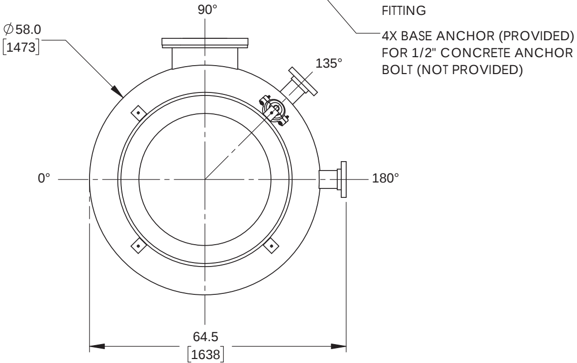
BOTTOM VIEW
